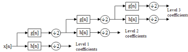
Fig. 2. Discrete wavelet transform
