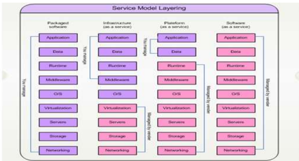
Figure 2. Service Model Layering 12 .
