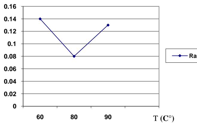
Figure 8. Roughness change with respect to temperature.
