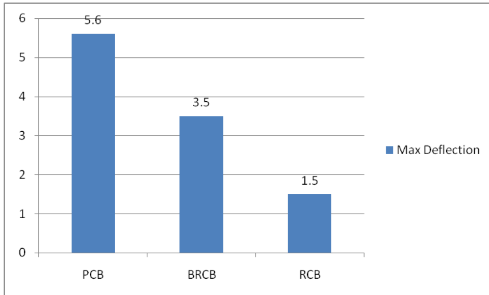
Figure.9 –Maximum Deflection for different type of Beam
