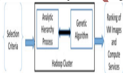
Fig.2. Overview of Hybrid Multi-goal Optimization Heuristic Method (HMOHM) Approach.
